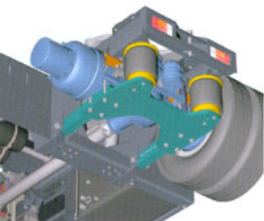
3-D view of rear axle/air suspension
